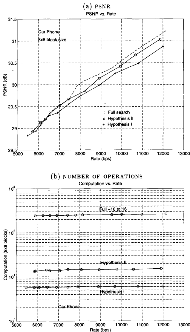
Figure 3. Performance of the probabilistic models in terms of PSNR and number of computations relative to the FS-BMA: CAR PHONE.
