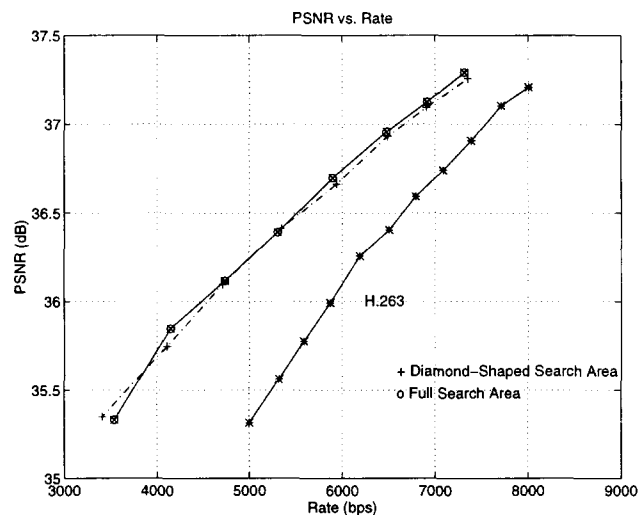
Figure 4. Performance comparison between the proposed video coder and Telenor's TMN5 (using all advanced options) for the test sequence MISS AMERICA at very low bit rates.
