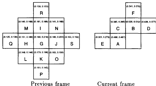
Figure 2. Average correlation values ( c_x, c_y ) of the ROS motion vectors with the current one.
