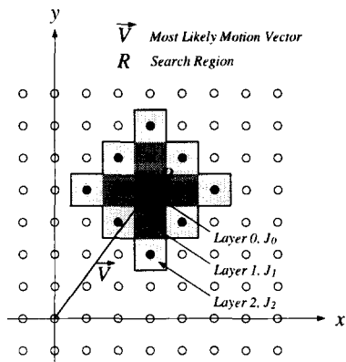
Figure 1. A diamond-shaped vector search area.
