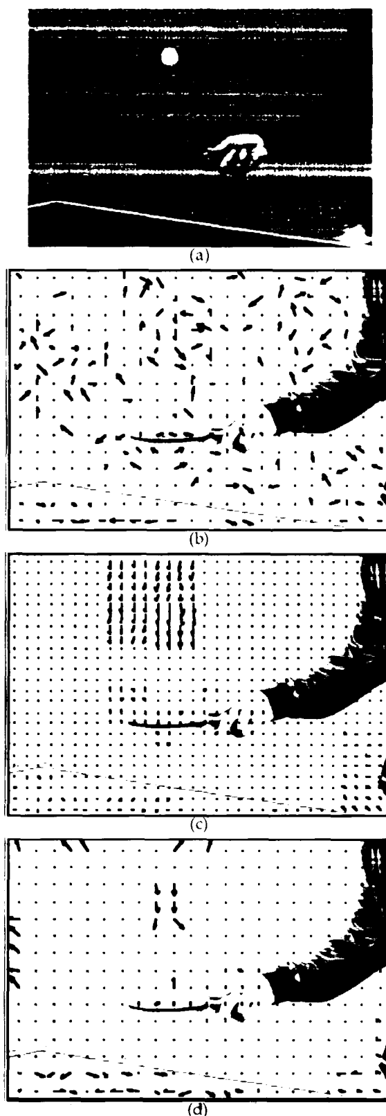
Fig 1: Motion estimates for frame 2 of the Table Tennis sequence using different algorithms. (a) original frame (b) CtF (c) CtF-FBS (d) FtC-T(R)
