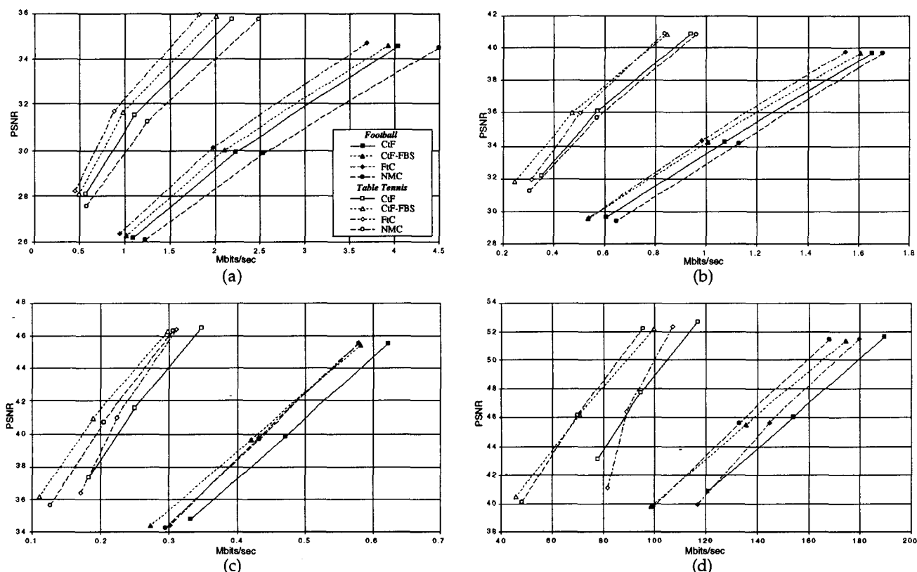
Fig 2: PSNR-rate curves for Football and Table Tennis for various resolutions. (a) 352x240 (b) 176x120 (c) 88x60 (d) 44x30
