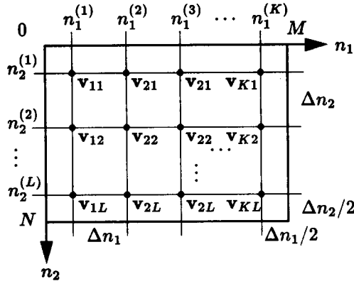
Figure 2: Initial placement of image vectors \mathbf{v}_{ij}
