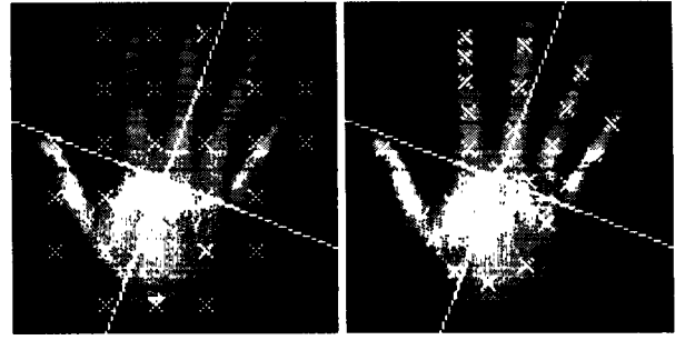
Figure 3: Initial and optimal image vectors with a non-zero attribute in a spatially segmented grey level image ( 11 \times 8 grid)
