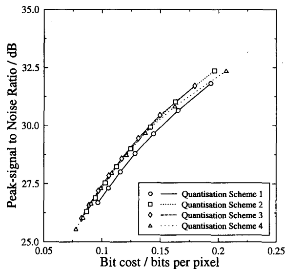
Figure 4: Performance of the 3D-DCT lenticular-integral image coding scheme for several quantisation strategies.
