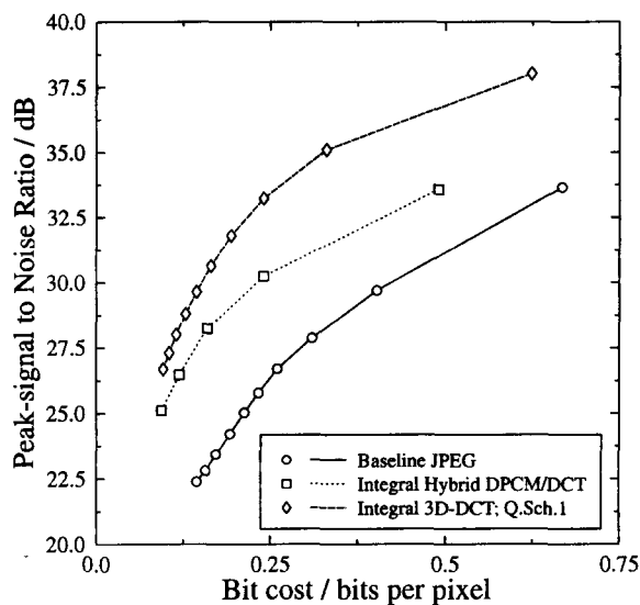
Figure 3: Performance of the 3D-DCT lenticular-integral image coding scheme, the hybrid DPCM/DCT scheme and baseline JPEG for compression of a greyscale integral 3D image.
