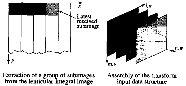
Figure 2: Assembly of 3D-DCT input data structure
