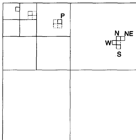
Significant Bitplane
