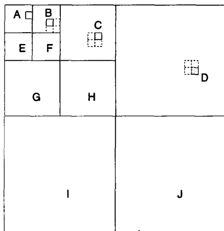
Current Bitplane
