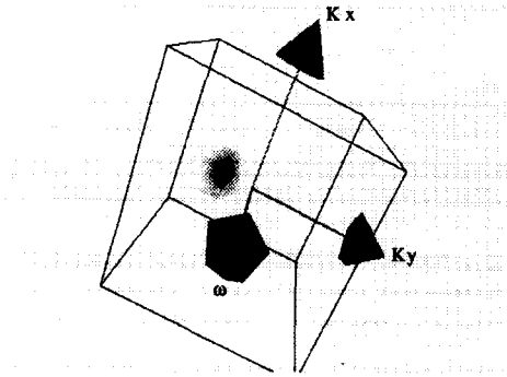
Figure 1. Galilean wavelet in velocity plane (1,0).
