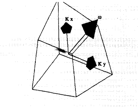
Figure 2. Galilean wavelet in velocity plane (1,0).
