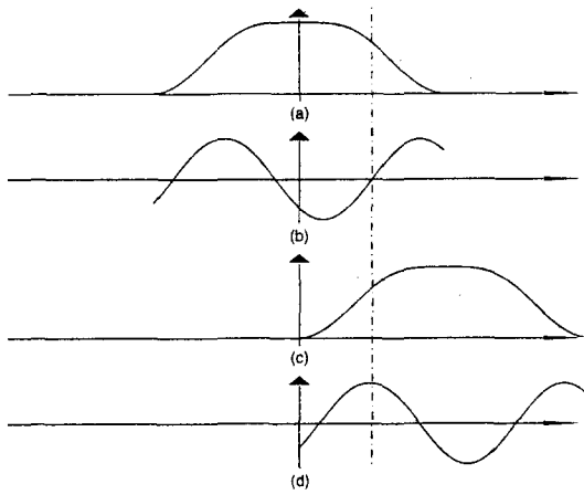
Fig. 1. Graphical proof of orthogonality. (a) Window w(x) . (b) Signal S(x) symmetric verifying (1). (c) Window in (a) translated of one step. (d) Signal S_1(x) antisymmetric around 1/2 .
