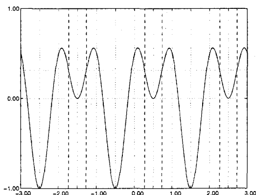
Fig. 5. Graphical explanation of the self-orthogonality condition. The product of two functions enjoying the same symmetries is symmetric both around \pm 1/2 and periodic with period 2. Because of this, the samples of the product w(x)w(x-2) relative to the instants shown with dashed lines "see" the same value. Note that the set of such instants can be written as x_0 + 2\mathbb{Z} \cup (1-x_0) + 2\mathbb{Z} . In the figure x_0 = 0.27 .
