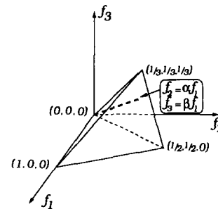
Figure 1. Trifrequency space showing the region used for feature calculations. The frequency axes, f_1 , f_2 , and f_3 are normalised by the Nyquist frequency.
