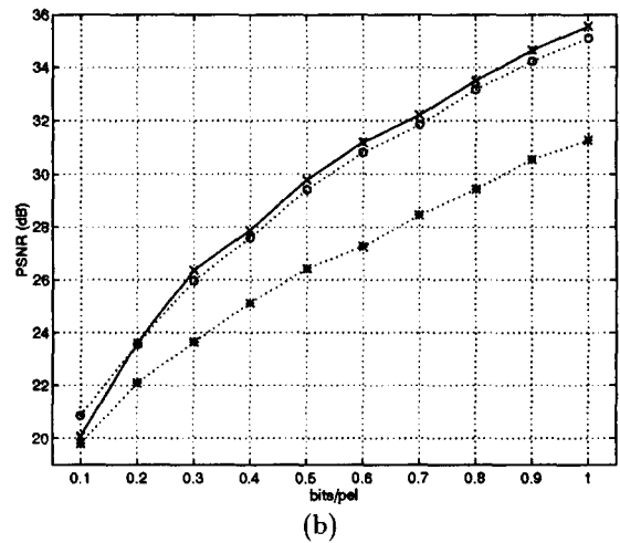
Figure 2. FB 24_12_12 ( \times ), WL 25_21_7 ( \circ ), and FB 7_11_5 (*). (a) "Lenna" and (b) "Barbara".
