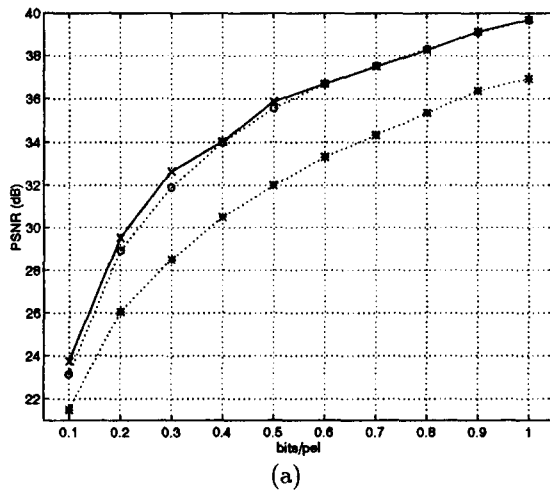
Figure 2. FB 24_12_12 ( \times ), WL 25_21_7 ( \circ ), and FB 7_11_5 (*). (a) "Lenna" and (b) "Barbara".
