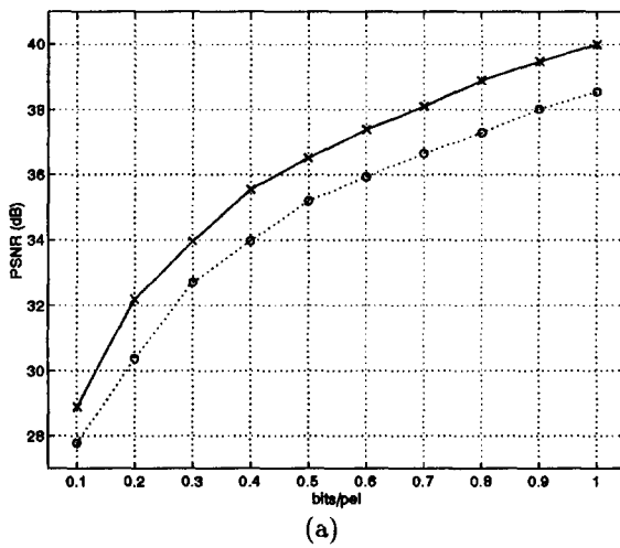
Figure 1. FB 33_25_21_7 WSI ( \times ), and FB 33_25_21_7 WOI ( \circ ). (a) "Lenna" and (b) "Barbara".
