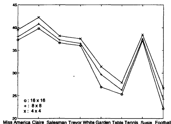
Figure 1. The trade-off between the block size and the picture quality.
