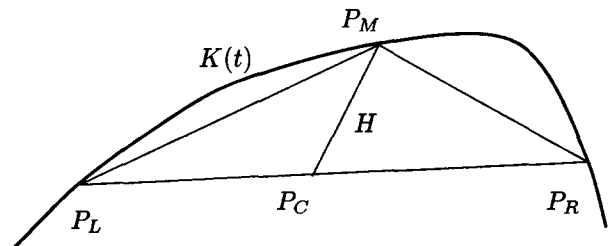
Fig. 7. Corner Detection
