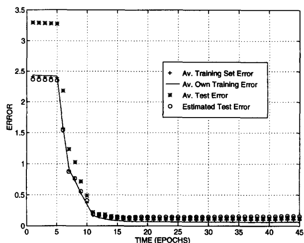
Figure 4: Overtraining scenario with a large network and near optimal regularization (weight decay). The data set and the networks are the same as in figure Fig. 3. Note that both the estimated and the measured test error suggest so stop training around itr = 15 . Note also that like in the previous neuroimaging case, figures Fig. 1 - Fig. 2, the overall level of test error is lower in this case, suggesting that careful control of the weight decay may be more efficient than early stop in optimizing generalization.
