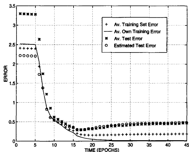
Figure 3: Overtraining scenario with large network and small regularization (weight decay). The data set is the wellknown sunspot prediction problem. The data set comprises N = 209 examples and an additional test set contains 35 examples. The Bootstrap ensemble had Q = 15 members. Each member is a feed-forward net with 12 input units, 8 hidden sigmoid units, and one output unit. The networks were trained by conventional backprop ( 1 \leq itr \leq 5 ), and by a second order pseudo Newton scheme ( 6 \leq itr \leq 45 ). The goal is to predict the noisy time series one-step-ahead based on a lag space of 12 previous values of the time series. In this run the network was only slightly regularized by weight decay. Errors are reported as normalized by the total variance of the series. Note that both the estimated and the measured test error suggest to stop training at around itr = 12 .
