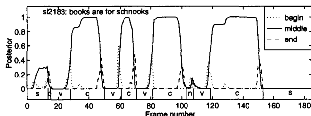
Figure 1. State posterior probabilities P(\pi_i|x, \mathcal{M}) for the three states in the consonant submodel for test sentence "si2183". The broad class segmentation is shown at the bottom of the plot.
