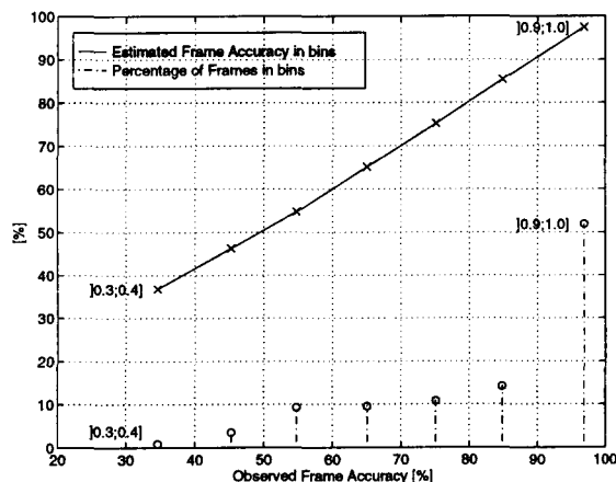
Figure 2. Solid line: Average label posterior probability of winning class \bar{P}(y^*|x, \mathcal{M}) ranked into 7 equally spaced bins and plotted as function of the observed frame accuracy in these bins. Dashed line: Percentage of frames falling into the 7 bins located at the corresponding observed frame accuracies.
