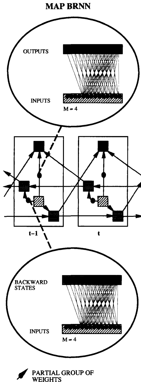
Figure 2. Bidirectional recurrent neural network structure (BRNN), with the state neurons split up into forward and backward state neurons, here with extensions for MAP forward probability estimation with the target class input coded in the first 4 channels
