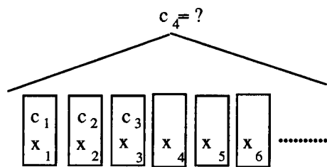
Figure 3. Visualization of the estimation problem for the MAP-forward probability
