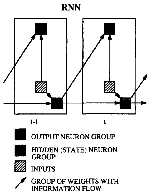
Figure 1. Regular (uni-directional) recurrent neural network structure (RNN)
