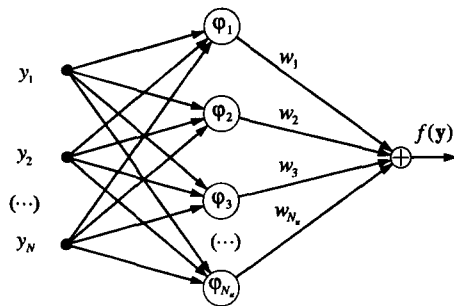
Figure 1. RBF network structure
