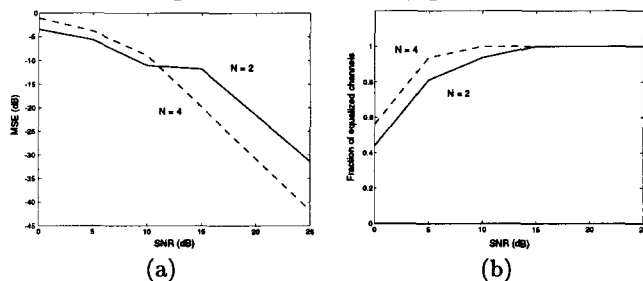
Figure 3. Random channel (a) Average MSE (b) Fraction of equalized channels
