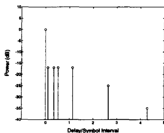
Figure 2. Power delay profile
