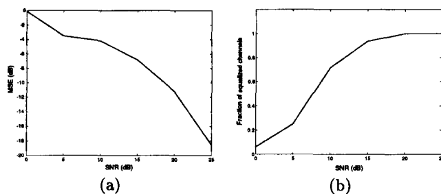
Figure 4. Time-varying random channel, N = 2 (a) Average MSE (b) Fraction of equalized channels
