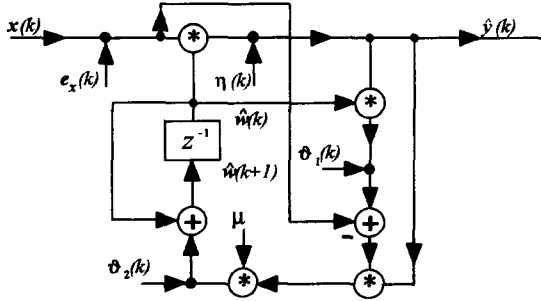
Fig. 1 The multiquantizer chain model of the PCA network
