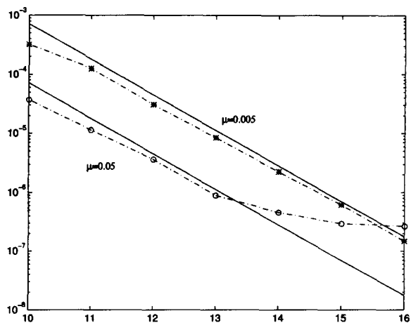
Fig. 2. A diagonal element of \tilde{P} versus the word-length of weights. Solid lines show the theoretical results.
