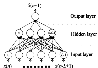
Figure 1: A predictive 2LFNN with L inputs, M hidden layer neurons, and a single output.
