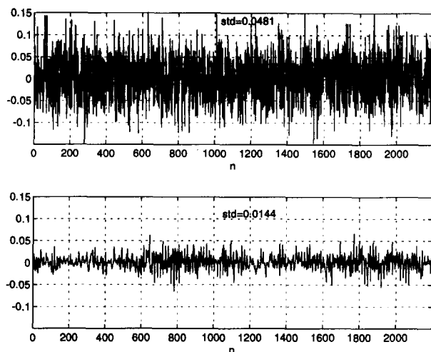
Figure 2. The error of reproduction of the distorted 1-D data; the upper curve - the state on the input to the network, the lower curve - the final state after noise reduction
