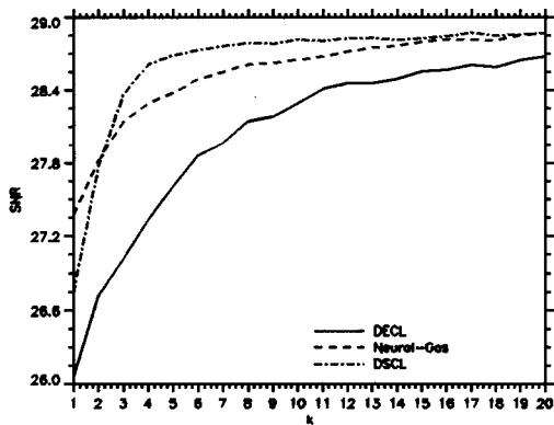
Figure 1-a. Plots of the SNR versus k for the three algorithms DSCL, DECL and "Neural-Gas" with the image "Lena" where k is related to the training steps
