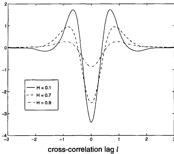
Figure 1: Cross-correlation \int_{-\infty}^{\infty} |u|^{2H(t)} \gamma_0(u-l) du , for \psi_0(t) , a Daubechies wavelet of regularity 2 (at scale a=1 ) and for three different values of the exponent H(t) .
