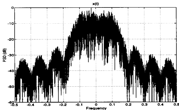
Figure 1. PSD of a quaternary CPFSK signal, x(t) , with h = 0.75
