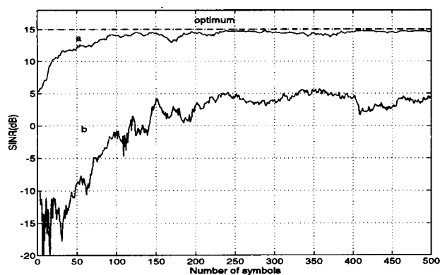
Figure 4. Interferences with different symbol rate: a) Proposed approach, b) Cross-SCORE.
