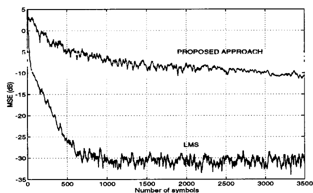
Figure 6. Time evolution of the MSE in the multipath scenario.
