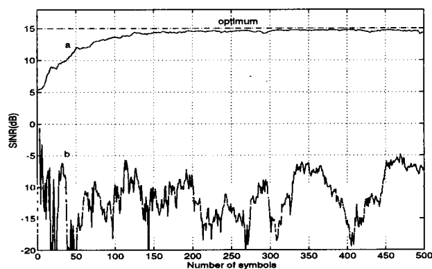
Figure 5. Interferences with the same symbol rate as the desired signal: a) Proposed approach with h = 2/3 , b) Cross-SCORE.
