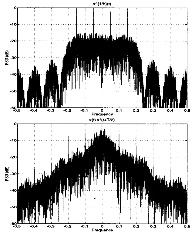
Figure 2. PSD of x^{1/h}(t) and z(t) = x(t)x^*(t + T/2)
