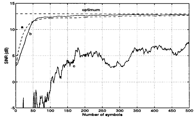
Figure 3. Time evolution of output SNR: a) Proposed approach with h = 2/3 , b) Proposed approach with h = 2/5 c) Cross-SCORE.
