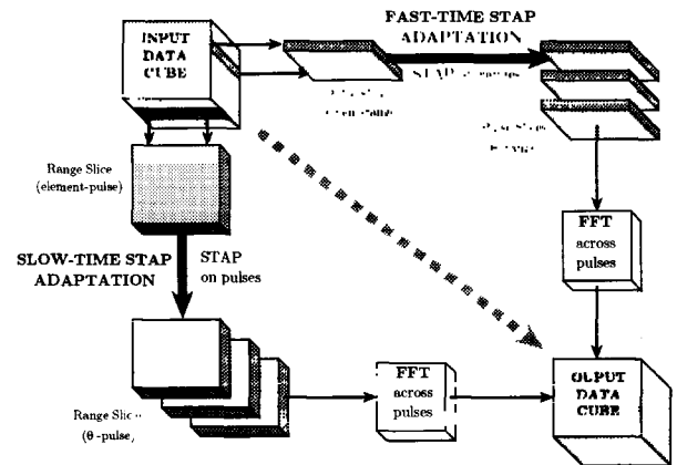
Figure 1. Fast- and slow-time STAP processing implementations.
