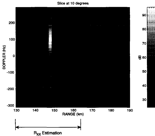
Figure 3. Range-Doppler plot obtained with single-constraint processing.
