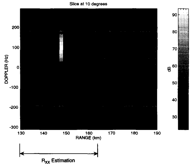
Figure 4. Range-Doppler plot obtained with multiple-constraint processing.
