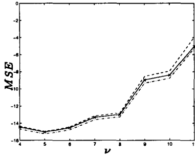
Figure 4: Dashed line: \mathcal{E}_U ; Solid line: \mathcal{E}_c ; Cross: \hat{\mathcal{E}} ; Dashdot: \mathcal{E}_m ; SNR = 20dB , r = 1(\text{BPSK}) , n = 8 .
