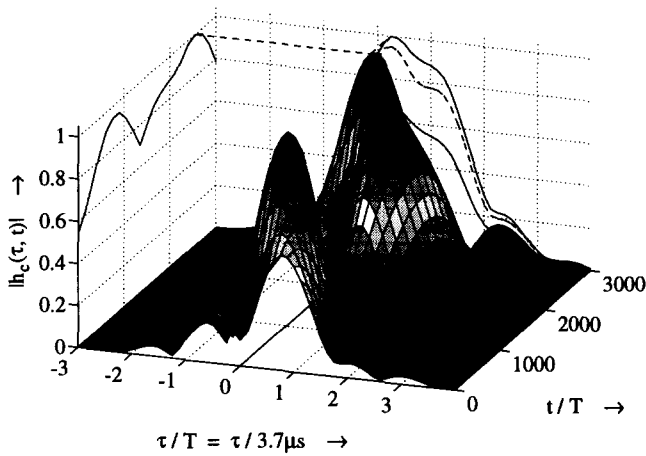
Figure 4: Impulse response of a Bad Urban channel
