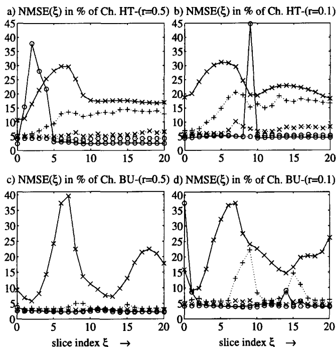
Figure 5: NMSE( \xi ) in % of TXK (solid) and EVI (dotted): “o”: \bar{S}/N = \infty , “x”: 10 dB, “+”: 7 dB
