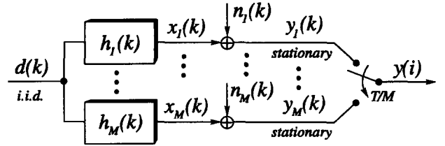
Figure 3: Stationary polyphase representation of y(i)
