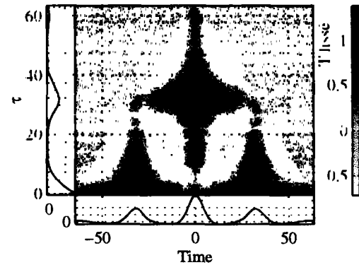
Figure 5. Smoothed time-product function \tilde{T}_{t,0}(\tau) for \omega = 0
