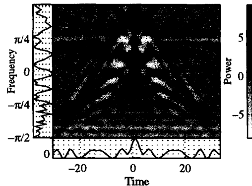
Figure 9. Optimal kernel distribution of "singauß"
