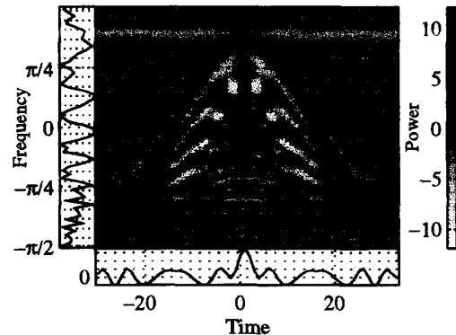
Figure 7. WVD of the signal "singauß"
