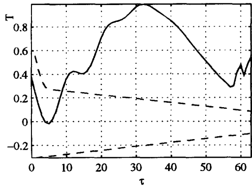
Figure 6. Estimation at t = 0 , \omega = 0 : \tilde{T}_{0,0}(\tau) (solid), thresholds (dashed)
