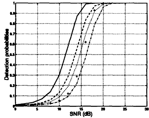
Figure 1: The average detection probabilities, K = 8 , P_F = 0.01 . The solid line is a performance bound, "--" is the new receiver, "-." is the correlator receiver, "..." is the MFIS receiver, and "+" is the energy detector.
