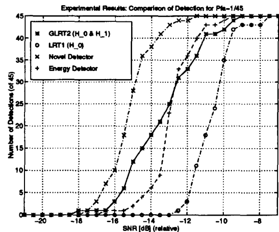
Figure 2: Experimental Results: Power of detection as a function of relative SNR.
