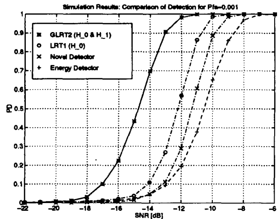
Figure 1: Simulation Results: Probability of detection as a function of SNR.
