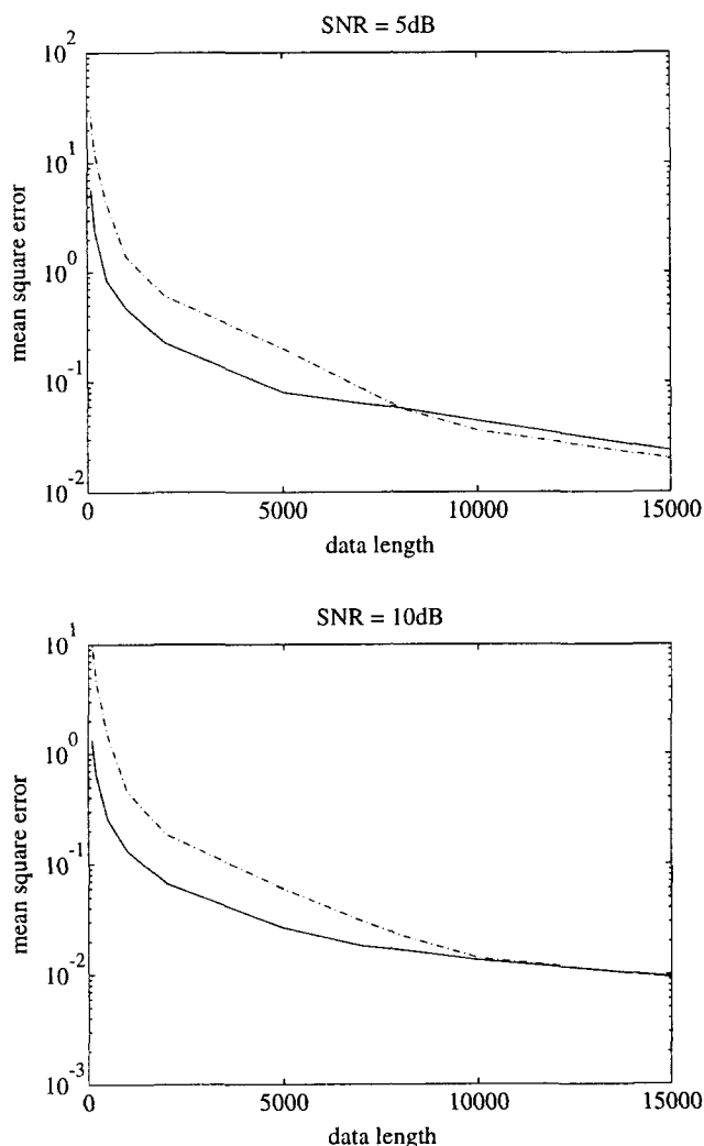
Figure 4: Comparison of the estimation errors using ESPRIT (solid lines) and VESPA (dash-dotted) at: (a) SNR = 5dB; (b) SNR = 10dB
