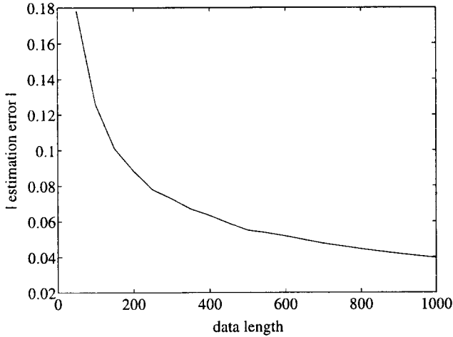
Figure 1: Cumulant estimation errors of a Gaussian process in terms of data length
