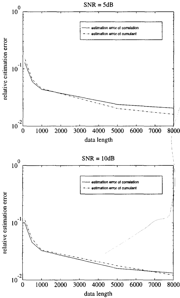
Figure 3: Influence of the suppression of Gaussian noise on the error of cumulant estimates of a distorted signal: (a) SNR = 5dB; (b) SNR = 10dB
