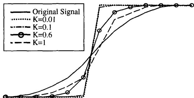
Figure 2. Providing edge enhancing capabilities to the median smoother via the family of estimators in (4). Smaller values of k induce increased edge sharpening capability. The median filter, corresponding to very large values of k , cannot modify the monotonic edge.
