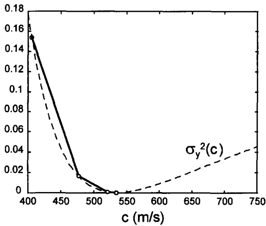
Figure 2. Example of the estimation of the propagation speed applying Newton method to \sigma_y^2(c) . The convergence is achieved in 5 steps for c=534 m/s with an initial guess of 408 m/s.
