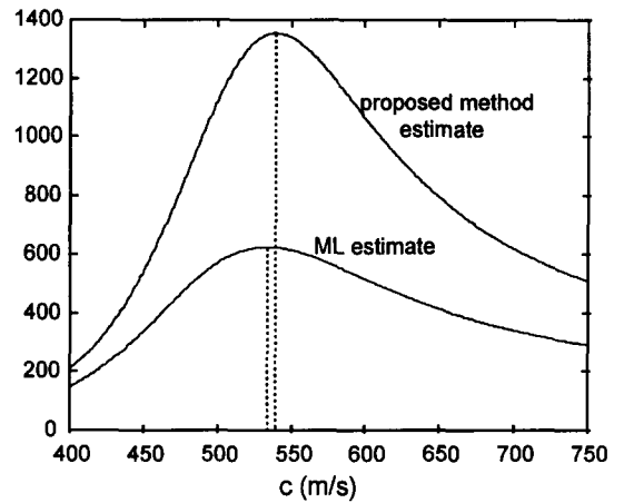
Figure 3. Comparison between the MLE and our estimate for 4 sensors and 64 samples. The true propagation speed is 535 m/s and the (S/N) = 30 dB. The ML estimates 533 m/s and our method does 539 m/s. The inverse of the output power is represented and units are linear.
