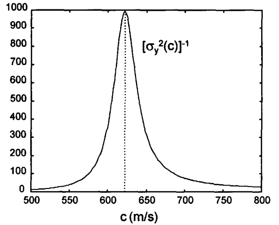
Figure 1. Inverse of the mean output power \sigma_y^2(c) for d/\lambda=1/5 , c=623 m/s and (S/N) = 30 dB. Units are linear.
