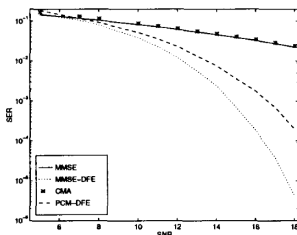
Figure 4: BER Performance
