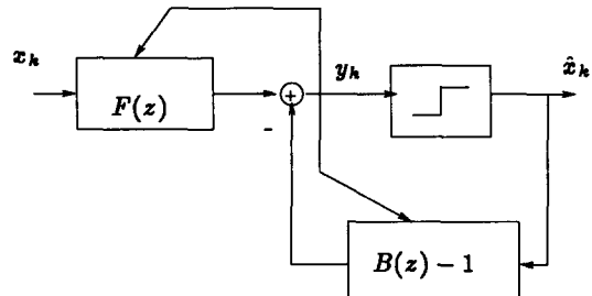
Figure 1: Schematic of CMA-DFE
