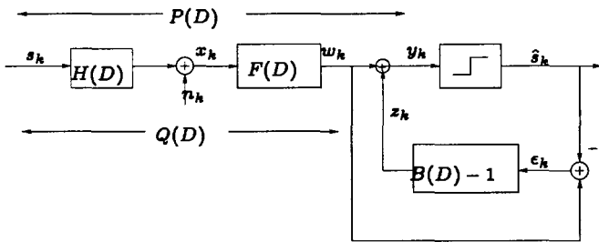
Figure 2: The Predictive structure of DFE
