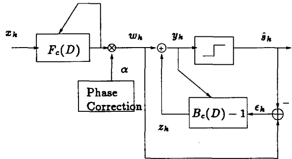
Figure 3: The Predictive CM-DFE
