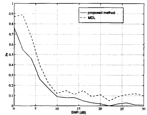
Figure 2: Probability of detection errors versus SNR for MDL and the proposed method, N=25 , L=12
