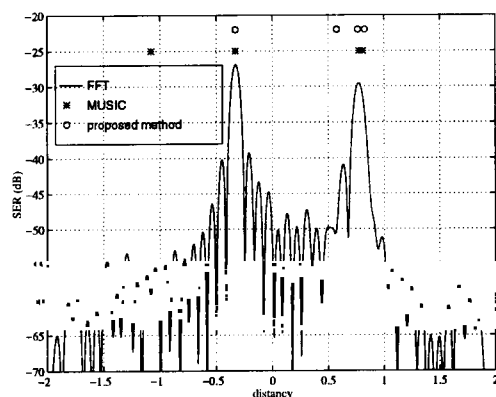
Figure 3: Simplified target : frequency band 8.2-10 GHz
