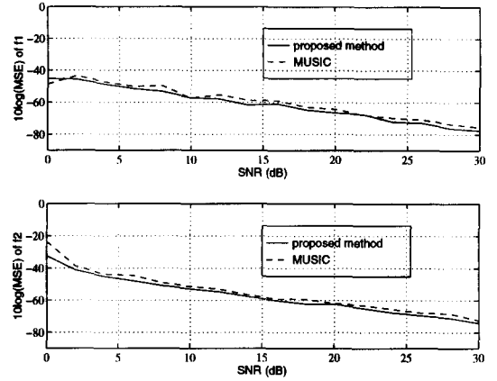
Figure 1: MSE's of the estimates of f_1 and f_2 versus SNR with MUSIC and with the proposed method, N=25 , L=12
