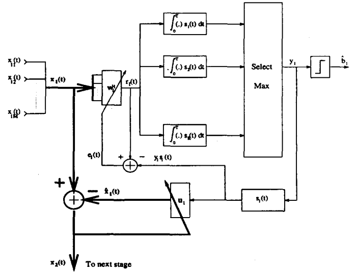
Figure 1. Block diagram of one stage of a Multielement interference canceller
