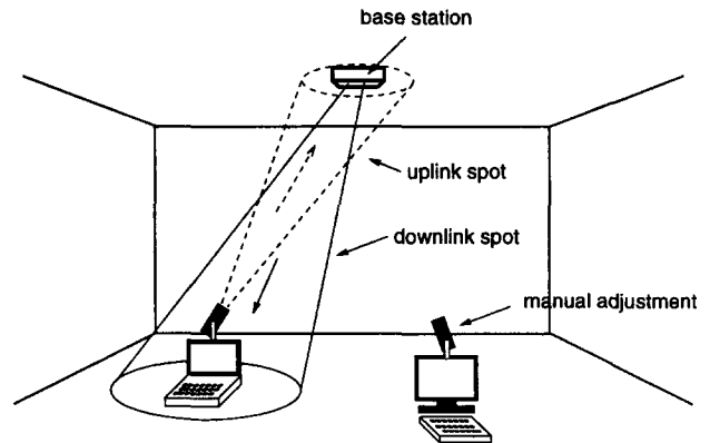
Figure 1. Proposed direct-beam system for large rooms providing placement flexibility.
