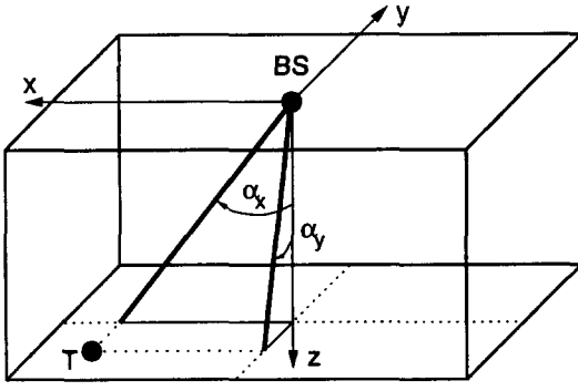
Figure 2. The DoA-estimation of terminals (T) contains the angles in the x - z -plane and the y - z -plane of an orthogonal x - y - z -reference system with base station (BS) in the coordinate-center.
