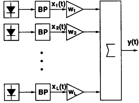
Figure 5. Beamformer with L elements
