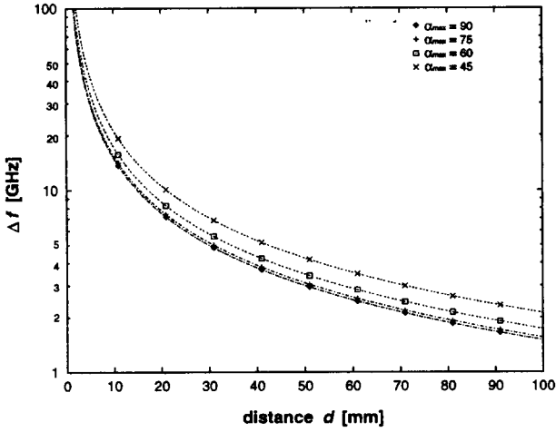
Figure 4. Required frequency difference as a function of d
