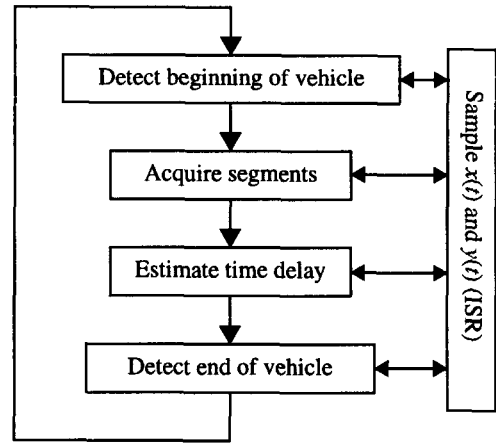
Figure 3. State machine running on the C31.
