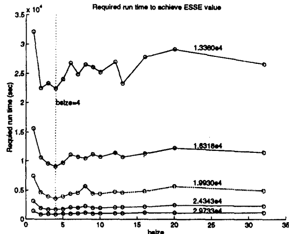
Figure 3. Epochs to reach a given ESSE vs. bunch size.
