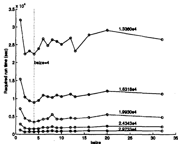
Figure 4. Time required to achieve a given ESSE vs. bunch size.
