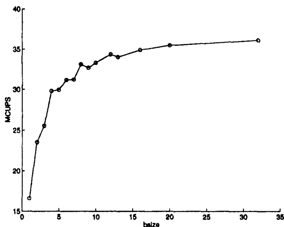
Figure 2. MCUPS vs. bunch size.
